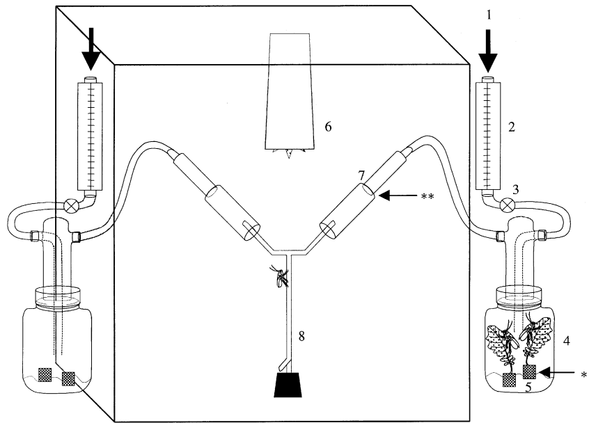
Figure 1 Schematic drawing of open Y-track olfactometer positioned in black box, with its open front covered by a black cloth during experiments. (1) Incoming clean air, (2) air flow control, (3) open/close valve, (4) glass bottle under a desk lamp (25 W), (5) square of wet oasis on a bottom of wet cotton, (6) lamp in black cylinder with red filter, (7) glass tube with gauze (arrow), (8) brass rod (diameter 4 mm, length to junction 13 cm) with extension at base for placing a male. Arrows indicate position of rubber septum in experiments I and III (*) and experiment II (**).
