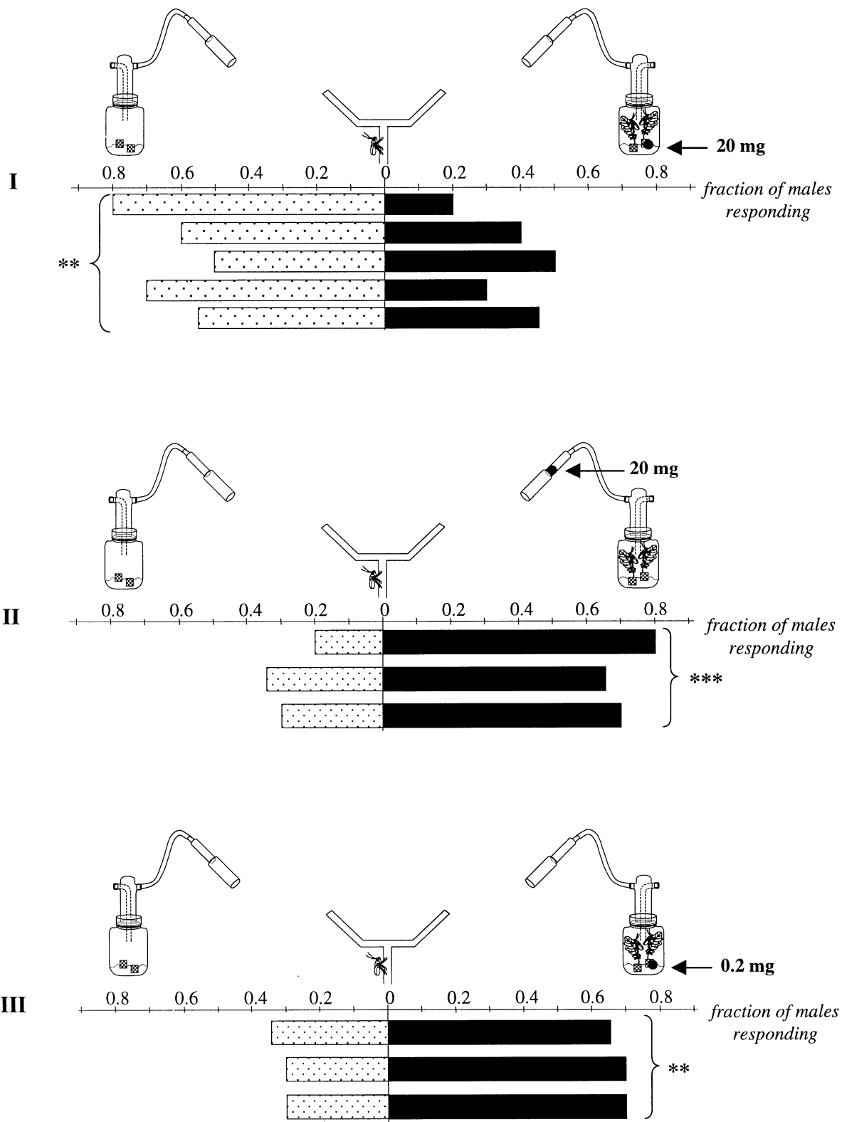
Figure 4 Y-track olfactometer tests. Odour sources tested: five females and a rubber septum, filled with 20 mg hexyl butanoate, (I) placed in the bottle with females, (II) placed downwind from the females, (III) filled with 0.2 mg hexyl butanoate, placed in the bottle with females (arrows indicate position of septa). Each bar represents one test with 20 males choosing. Preferences for odour sources were determined by using the two-sided binomial test for the mean results (after summing the replicates); ***0.01 < P < 0.001.
