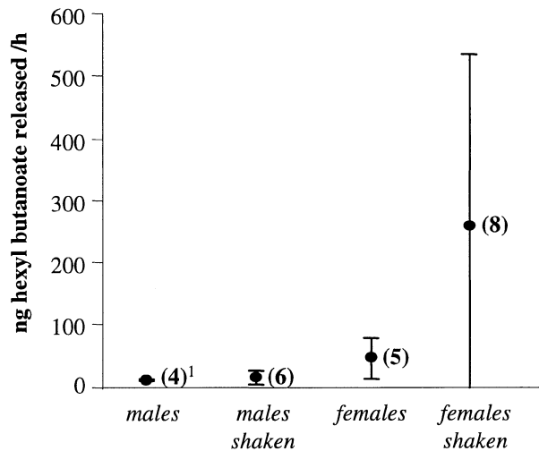
Figure 2 Amount ( \pm c.i.) of hexyl butanoate, released from five males or females in 1 h, in glass bottles that have been shaken or not. 1 Number of replicates. See text for further explanation.
